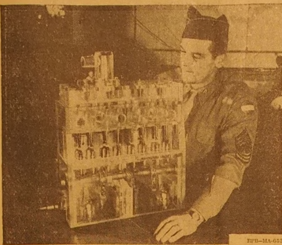
Visual clarity is obtained in this plastic model of a jeep engine built by M/Sgt. James Abbey of the Armored School, Fort Knox, Ky. Used in lectures in the Basic Engine Division of the school's Automotive Department, this transparent model enables the soldier-student to view the engine's interior parts while in motion.
